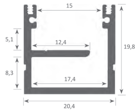
Insert V - dimensions drawing
