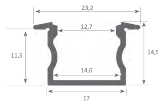
Insert P- dimensions drawing
