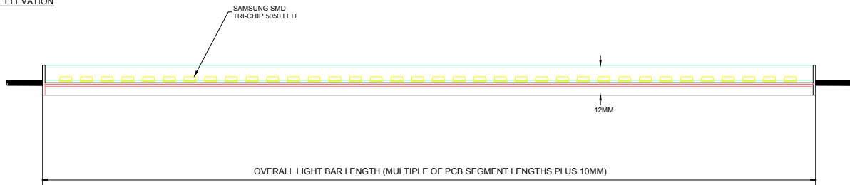
LED BAR - SIDE ELEVATION
