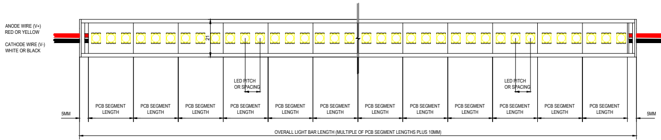
LED BAR - SIDE ELEVATION
