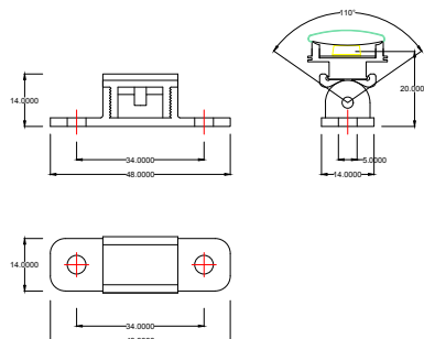
ANGLE ADJUSTABLE FIXING CLIP - 8.3mm pitch bar
