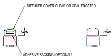
LED BAR - SECTION
