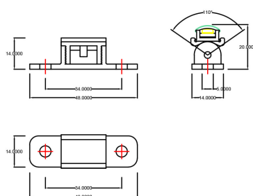
ANGLE ADJUSTABLE FIXING CLIP
