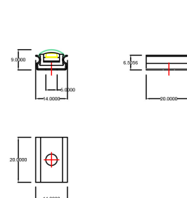
FLAT METAL FIXING CLIP
