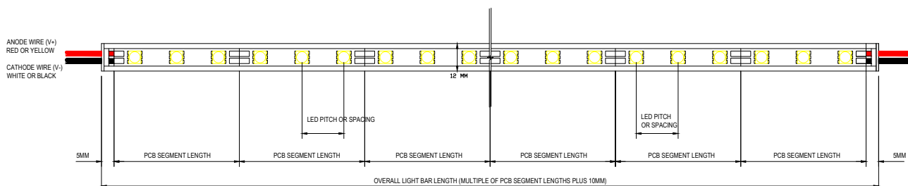
LED BAR - SIDE ELEVATION
