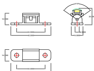
ANGLE ADJUSTABLE FIXING CLIP
