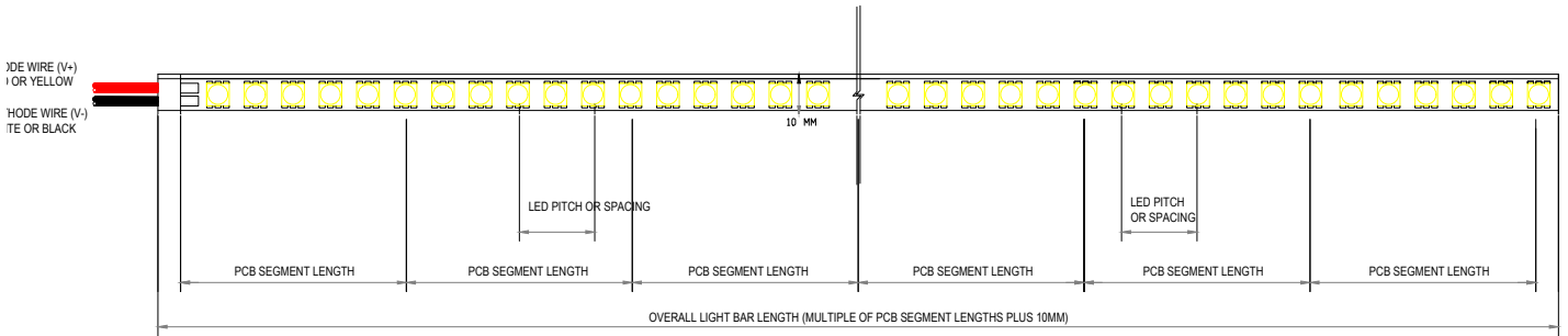
FLEXI STRIP ON BAR - PLAN
