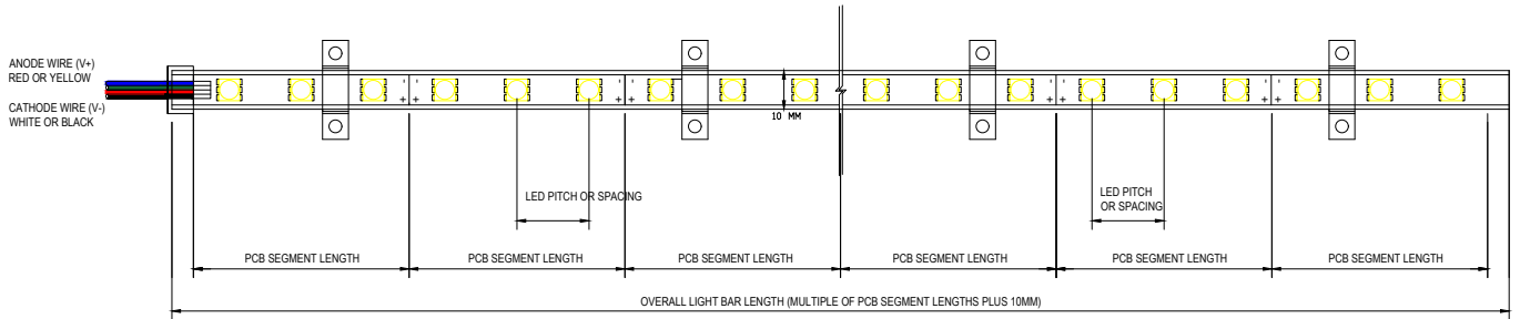
FLEXI STRIP - PLAN
